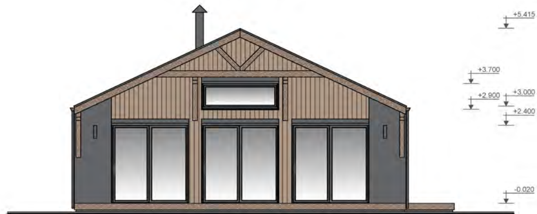
Facade 1. 1:75 (A-3)
